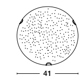
White Acrylic Diffuser LED 24 Watt 230 Volt 1680Lm 3000K-4000K-5500K IP20 D: 41 H: 9.5 cm
