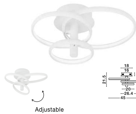
EMIL - 9349062 Dimmable Sandy White Aluminium & Acrylic LED 30 Watt 230 Volt 2300Lm 3000K IP20 D: 45 W: 35 H: 21.5 cm
